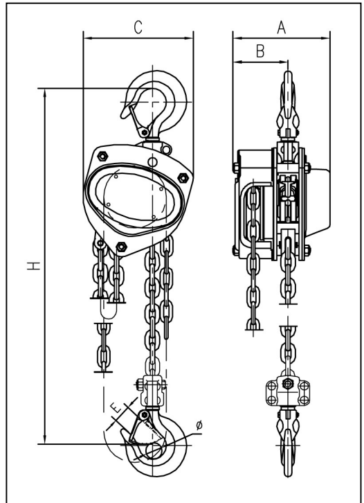
Fig. 1 Dimensioned sketch
