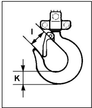
Fig 4 Load hook
